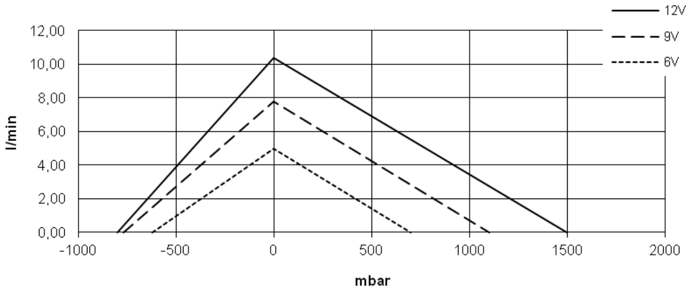
Type/Model: DC12/80SL
