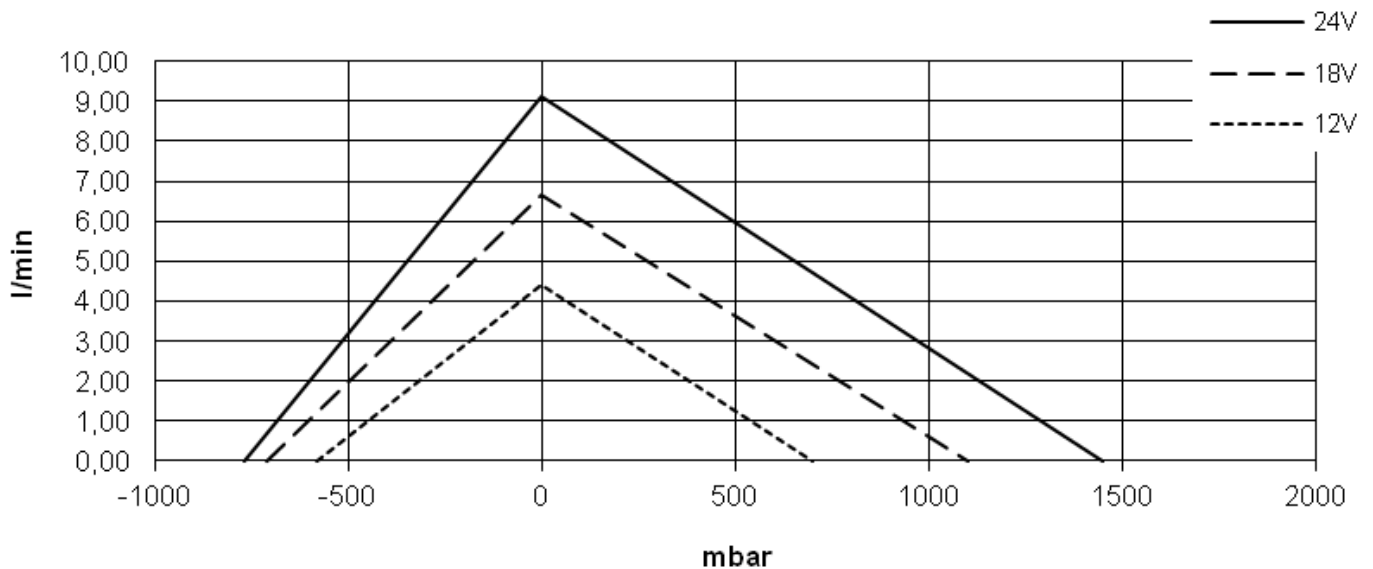
Type/Model: DC24/80SL
